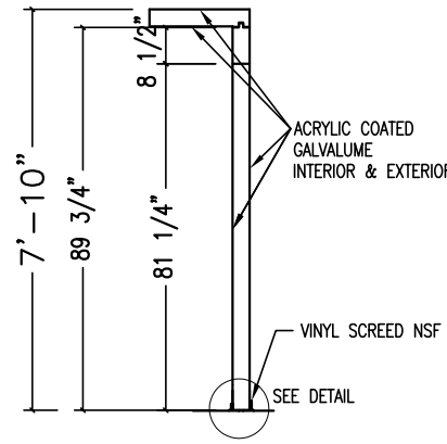
SECTIONAL VIEW AT G.D. OPG. FOR PASS-THRU DOOR
