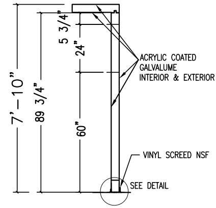
SECTIONAL VIEW AT OPG. FOR FIXED WINDOW
