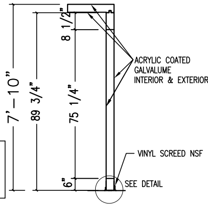
SECTIONAL VIEW AT G.D. OPG. FOR GLASS DOORS
